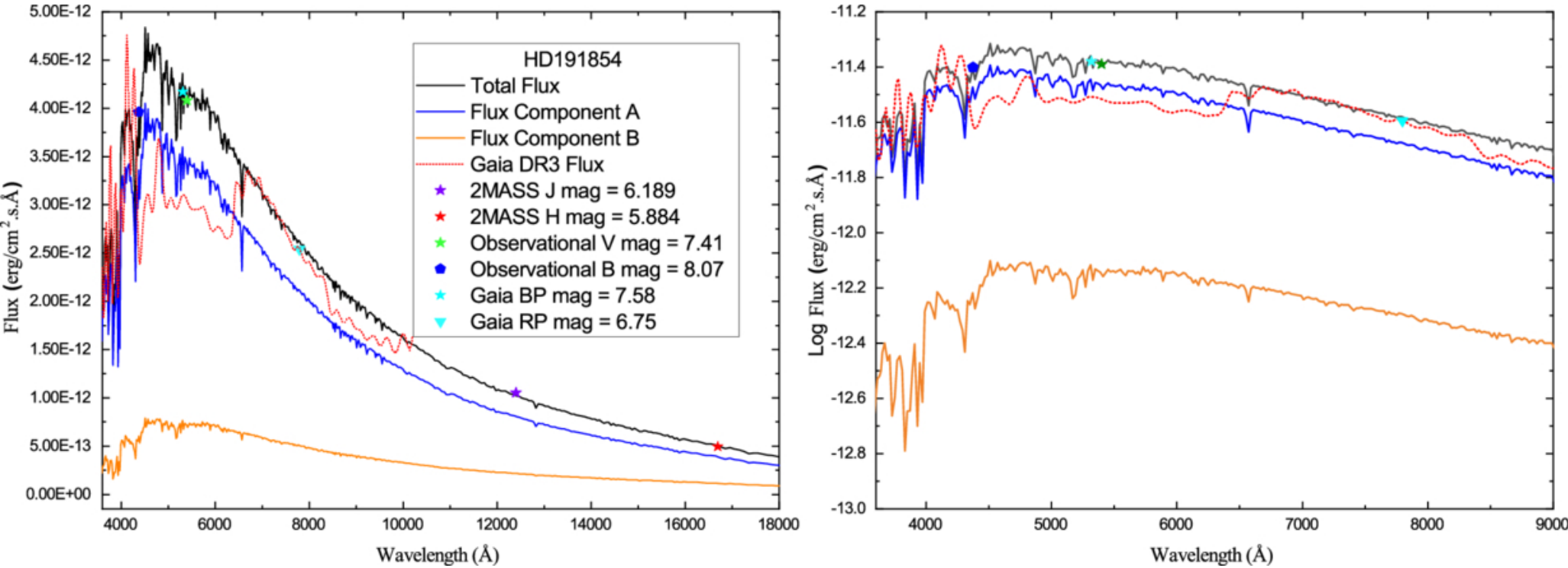
Figure 3. from Ahmad Abushattal et al 2025 Astron. J. 170 doi:10.3847/1538-3881/ae0582 https://dx.doi.org/10.3847/1538-3881/ae0582 © 2025. The Author(s). Published by the American Astronomical Society.
