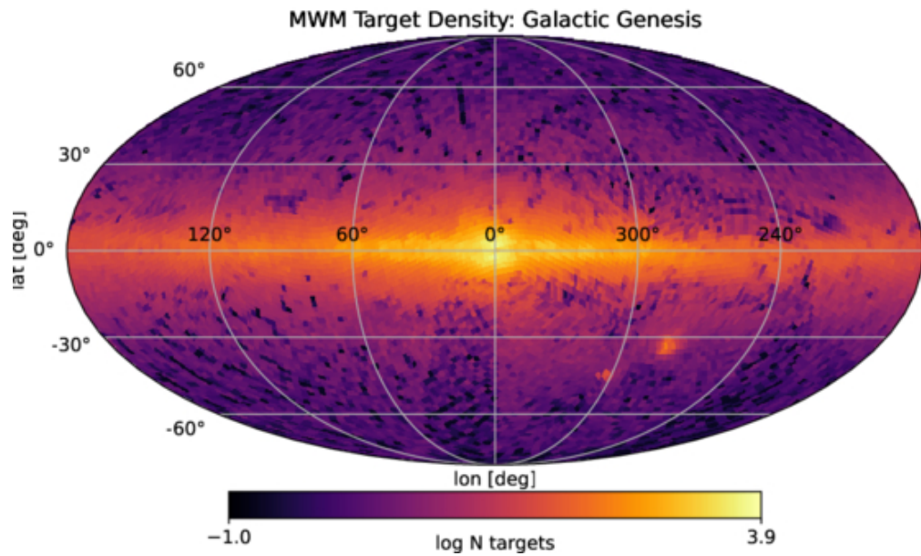
Figure 7. from Juna A. Kollmeier et al 2026 Astron. J. 171 doi:10.3847/1538-3881/ae0576 https://dx.doi.org/10.3847/1538-3881/ae0576 © 2025. The Author(s). Published by the American Astronomical Society.
