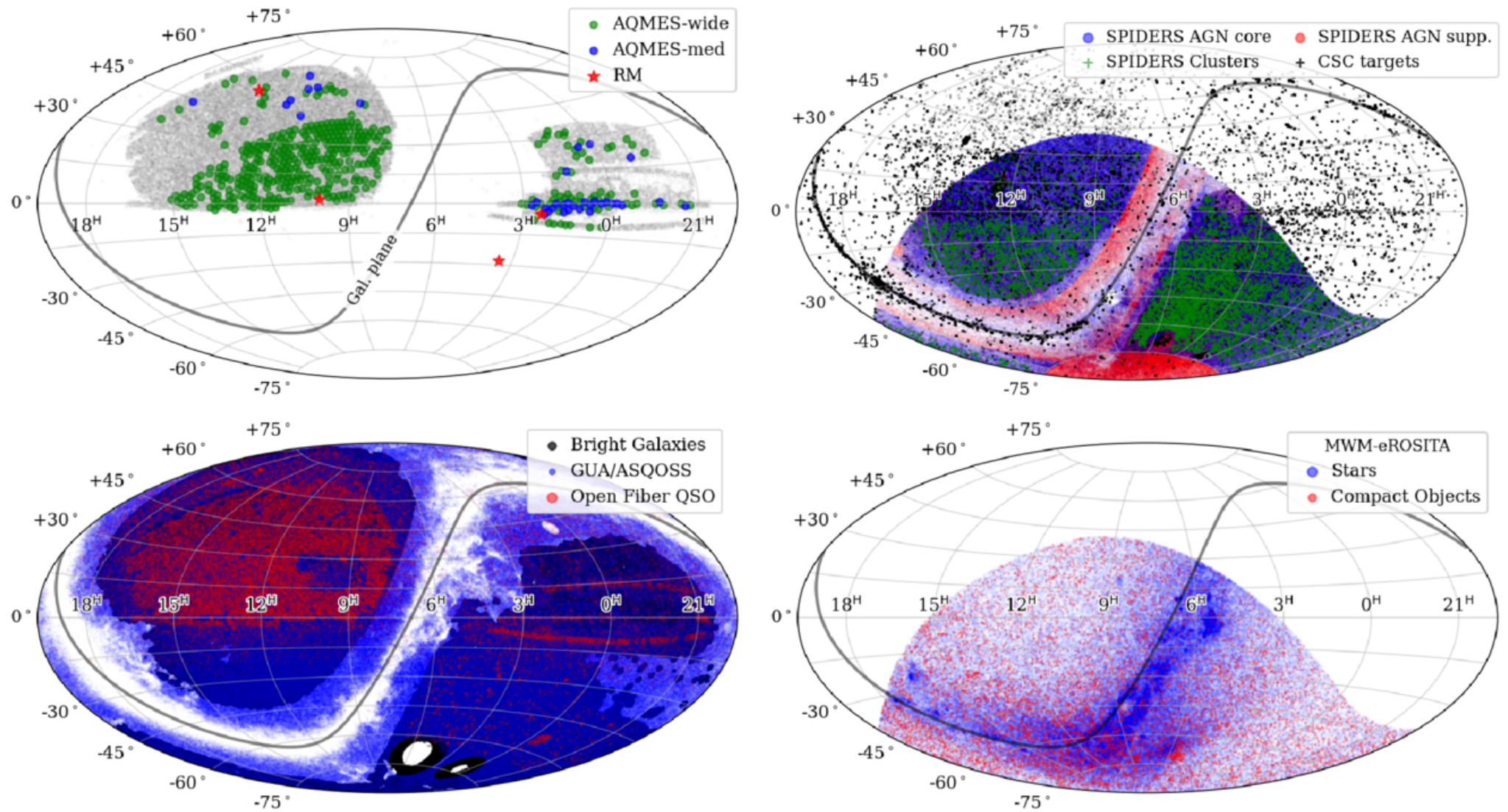
Figure 5. from Juna A. Kollmeier et al 2026 Astron. J. 171 doi:10.3847/1538-3881/ae0576 https://dx.doi.org/10.3847/1538-3881/ae0576 © 2025. The Author(s). Published by the American Astronomical Society.
