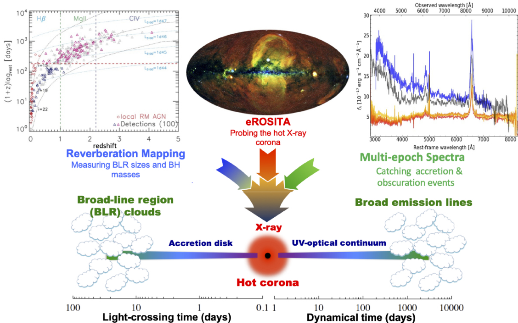
Figure 4. from Juna A. Kollmeier et al 2026 Astron. J. 171 doi:10.3847/1538-3881/ae0576 https://dx.doi.org/10.3847/1538-3881/ae0576 © 2025. The Author(s). Published by the American Astronomical Society.
