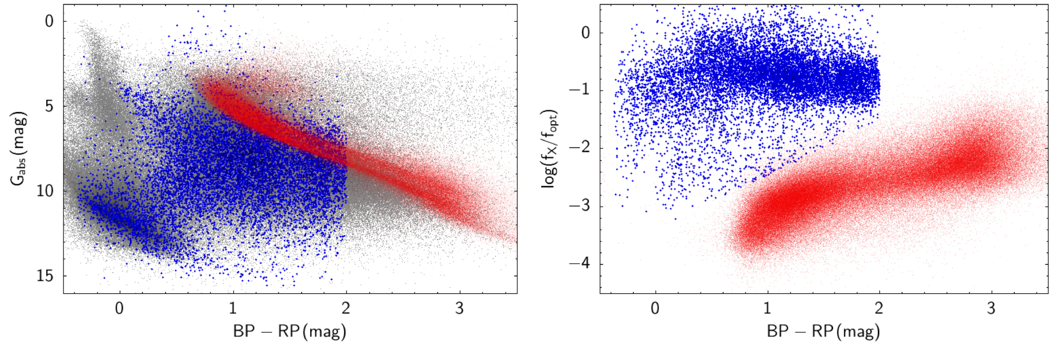
Figure 11. from Juna A. Kollmeier et al 2026 Astron. J. 171 doi:10.3847/1538-3881/ae0576 https://dx.doi.org/10.3847/1538-3881/ae0576 © 2025. The Author(s). Published by the American Astronomical Society.
