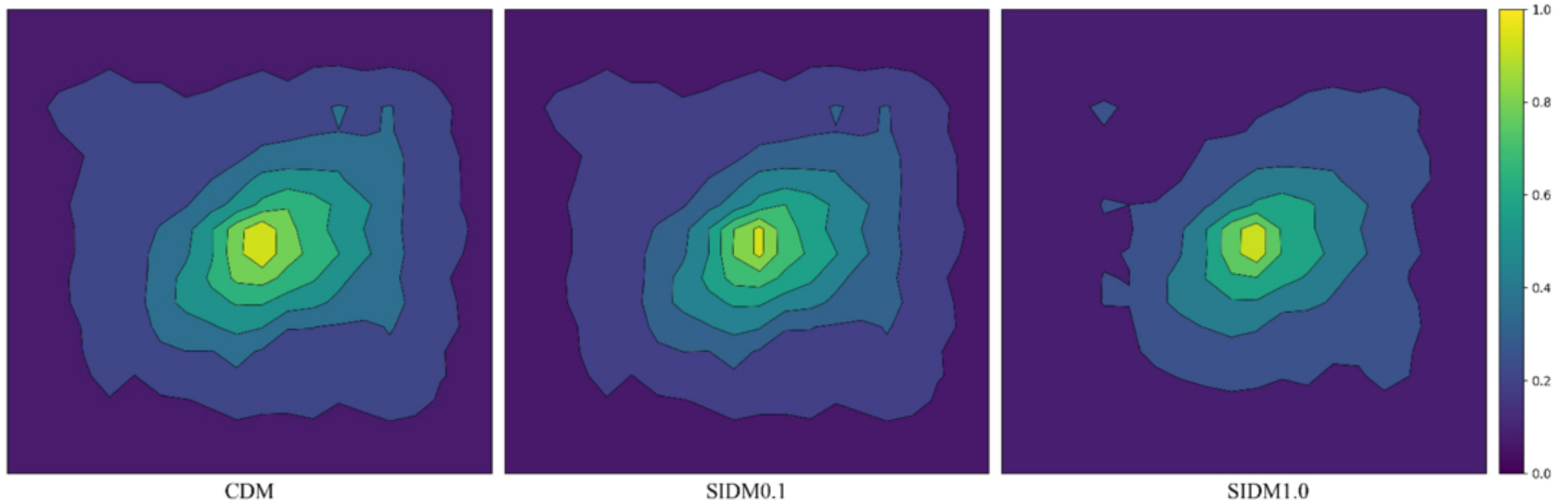
Figure 5. from Zhenyang Huang et al 2025 Astron. J. 170 doi:10.3847/1538-3881/ae0476 https://dx.doi.org/10.3847/1538-3881/ae0476 © 2025. The Author(s). Published by the American Astronomical Society.
