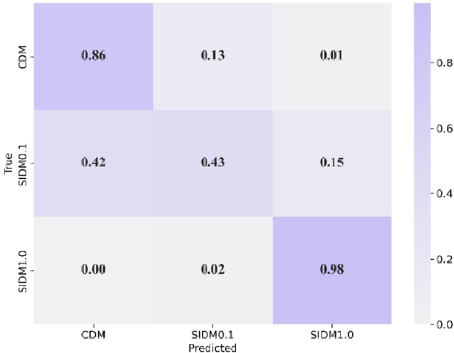
Figure 3. from Zhenyang Huang et al 2025 Astron. J. 170 doi:10.3847/1538-3881/ae0476 https://dx.doi.org/10.3847/1538-3881/ae0476 © 2025. The Author(s). Published by the American Astronomical Society.
