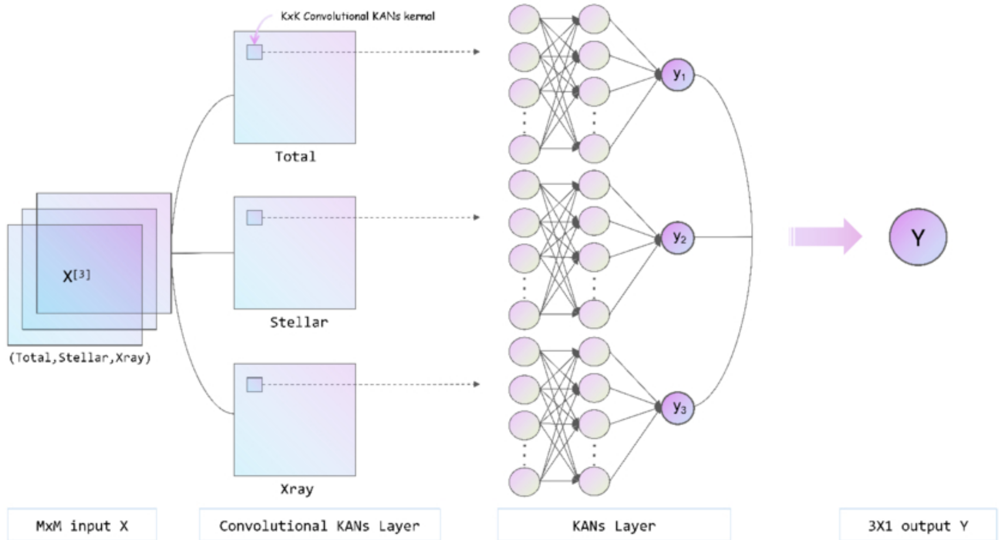
Figure 1. from Zhenyang Huang et al 2025 Astron. J. 170 doi:10.3847/1538-3881/ae0476 https://dx.doi.org/10.3847/1538-3881/ae0476 © 2025. The Author(s). Published by the American Astronomical Society.
