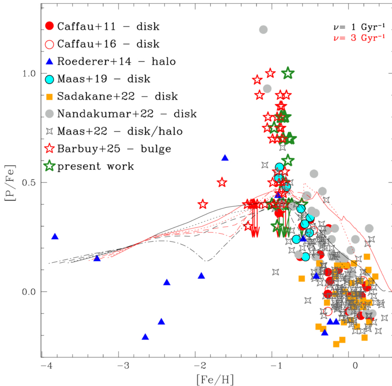
Figure 3. from Beatriz Barbuy et al 2025 Astron. J. 170 doi:10.3847/1538-3881/ae046b https://dx.doi.org/10.3847/1538-3881/ae046b © 2025. The Author(s). Published by the American Astronomical Society.
