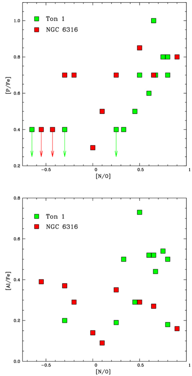
Figure 2. from Beatriz Barbuy et al 2025 Astron. J. 170 doi:10.3847/1538-3881/ae046b https://dx.doi.org/10.3847/1538-3881/ae046b © 2025. The Author(s). Published by the American Astronomical Society.
