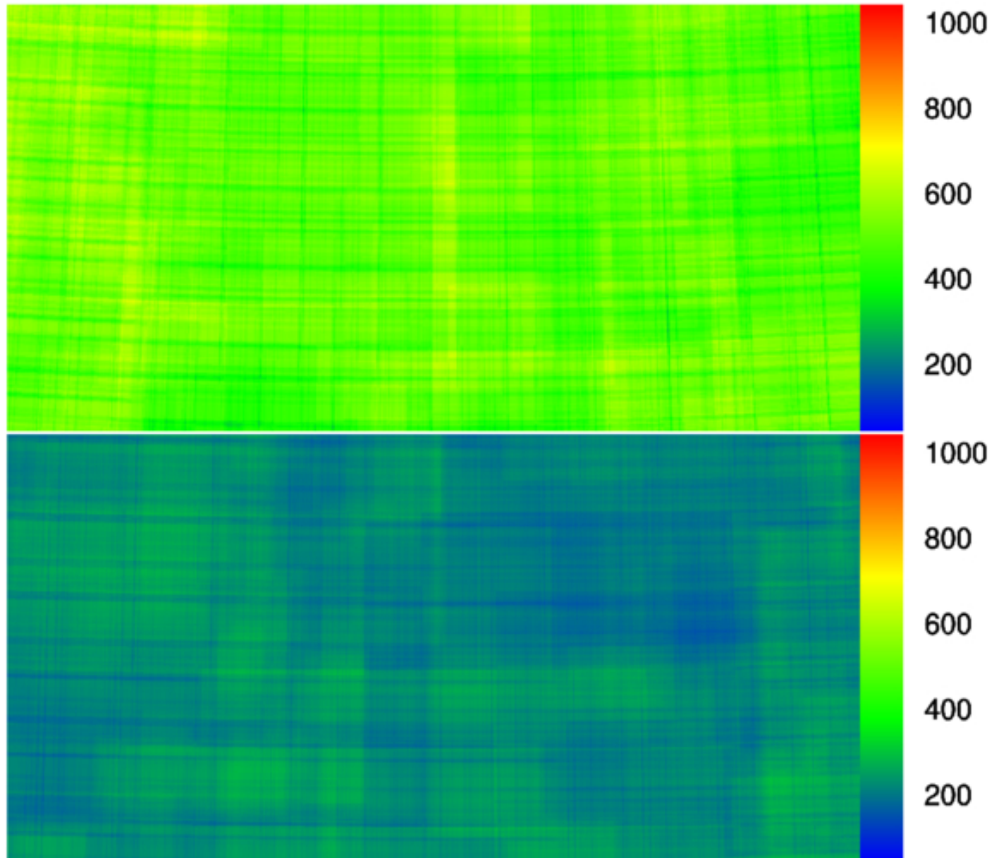
Figure 8. from Stephen Gwyn et al 2025 Astron. J. 170 doi:10.3847/1538-3881/ae03ab https://dx.doi.org/10.3847/1538-3881/ae03ab © 2025. The Author(s). Published by the American Astronomical Society.
