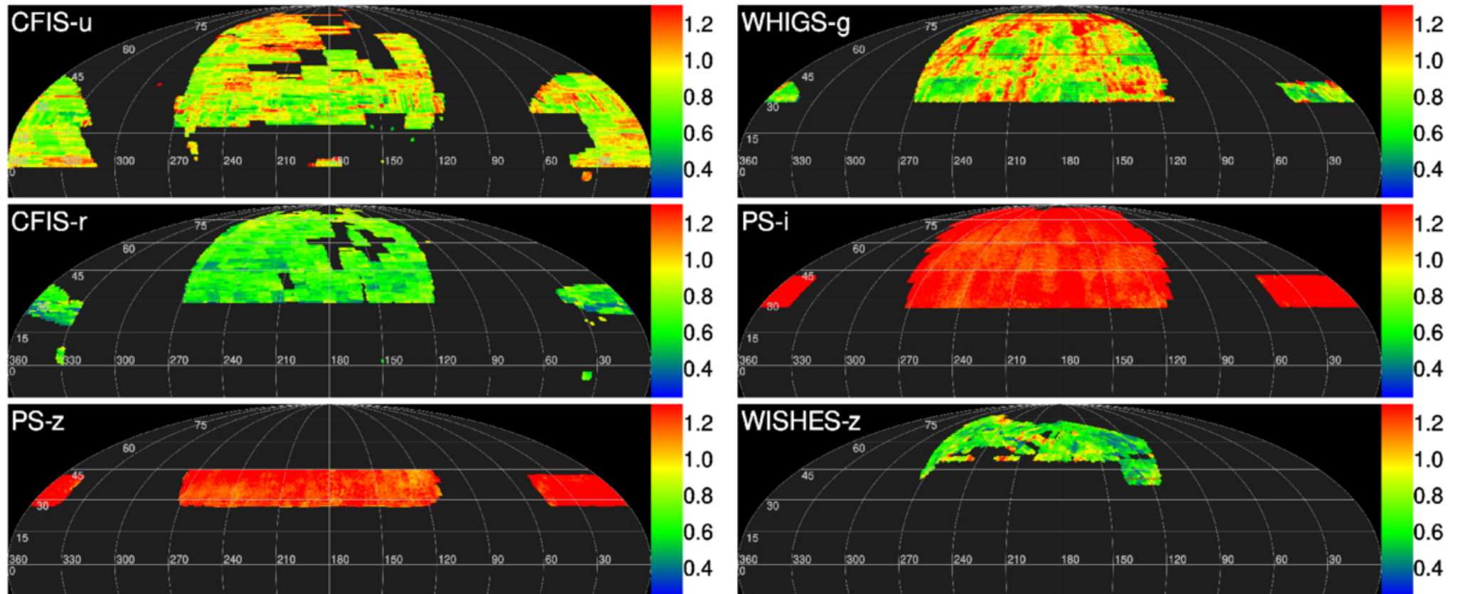
Figure 5. from Stephen Gwyn et al 2025 Astron. J. 170 doi:10.3847/1538-3881/ae03ab https://dx.doi.org/10.3847/1538-3881/ae03ab © 2025. The Author(s). Published by the American Astronomical Society.
