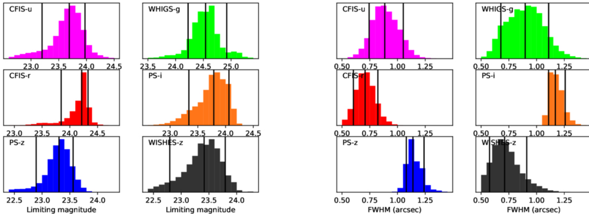
Figure 4. from Stephen Gwyn et al 2025 Astron. J. 170 doi:10.3847/1538-3881/ae03ab https://dx.doi.org/10.3847/1538-3881/ae03ab © 2025. The Author(s). Published by the American Astronomical Society.
