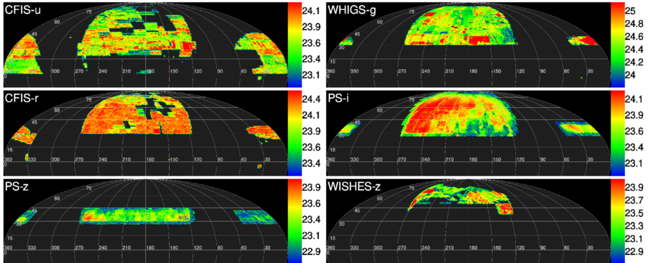
Figure 3. from Stephen Gwyn et al 2025 Astron. J. 170 doi:10.3847/1538-3881/ae03ab https://dx.doi.org/10.3847/1538-3881/ae03ab © 2025. The Author(s). Published by the American Astronomical Society.
