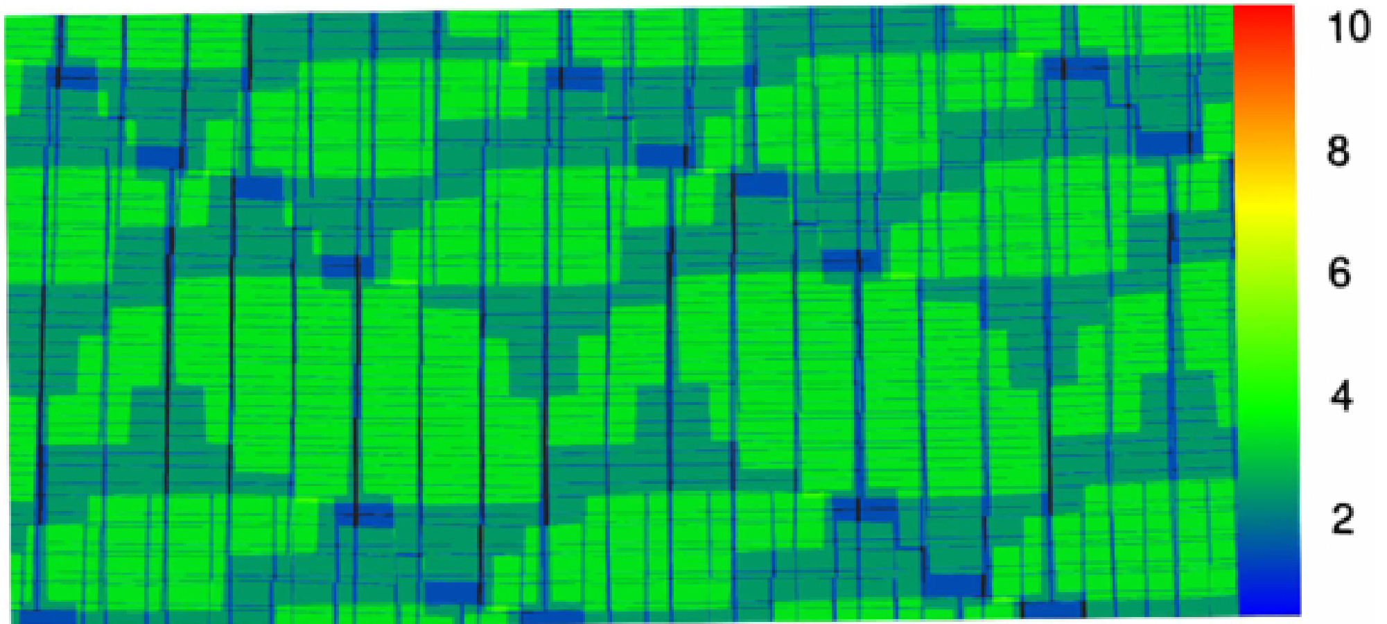
Figure 10. from Stephen Gwyn et al 2025 Astron. J. 170 doi:10.3847/1538-3881/ae03ab https://dx.doi.org/10.3847/1538-3881/ae03ab © 2025. The Author(s). Published by the American Astronomical Society.
