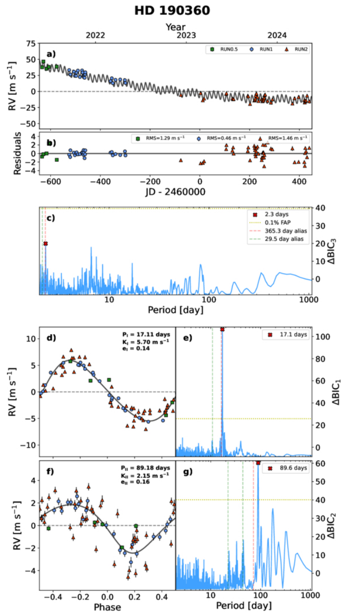
Figure 9. Blind RVSearch results for stars with known long-period companions. from Arvind F. Gupta et al 2025 Astron. J. 170 doi:10.3847/1538-3881/ae0339 https://dx.doi.org/10.3847/1538-3881/ae0339 © 2025. The Author(s). Published by the American Astronomical Society.
