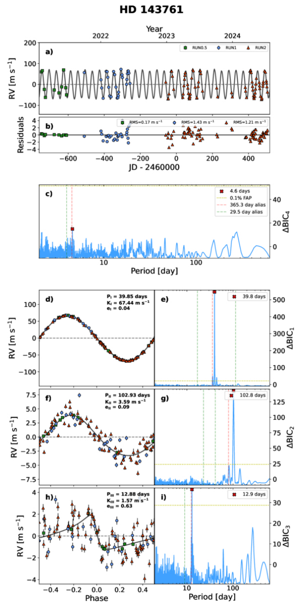
Figure 8. RVSearch results for stars with no known long-period companions. No trend allowed. from Arvind F. Gupta et al 2025 Astron. J. 170 doi:10.3847/1538-3881/ae0339 https://dx.doi.org/10.3847/1538-3881/ae0339 © 2025. The Author(s). Published by the American Astronomical Society.
