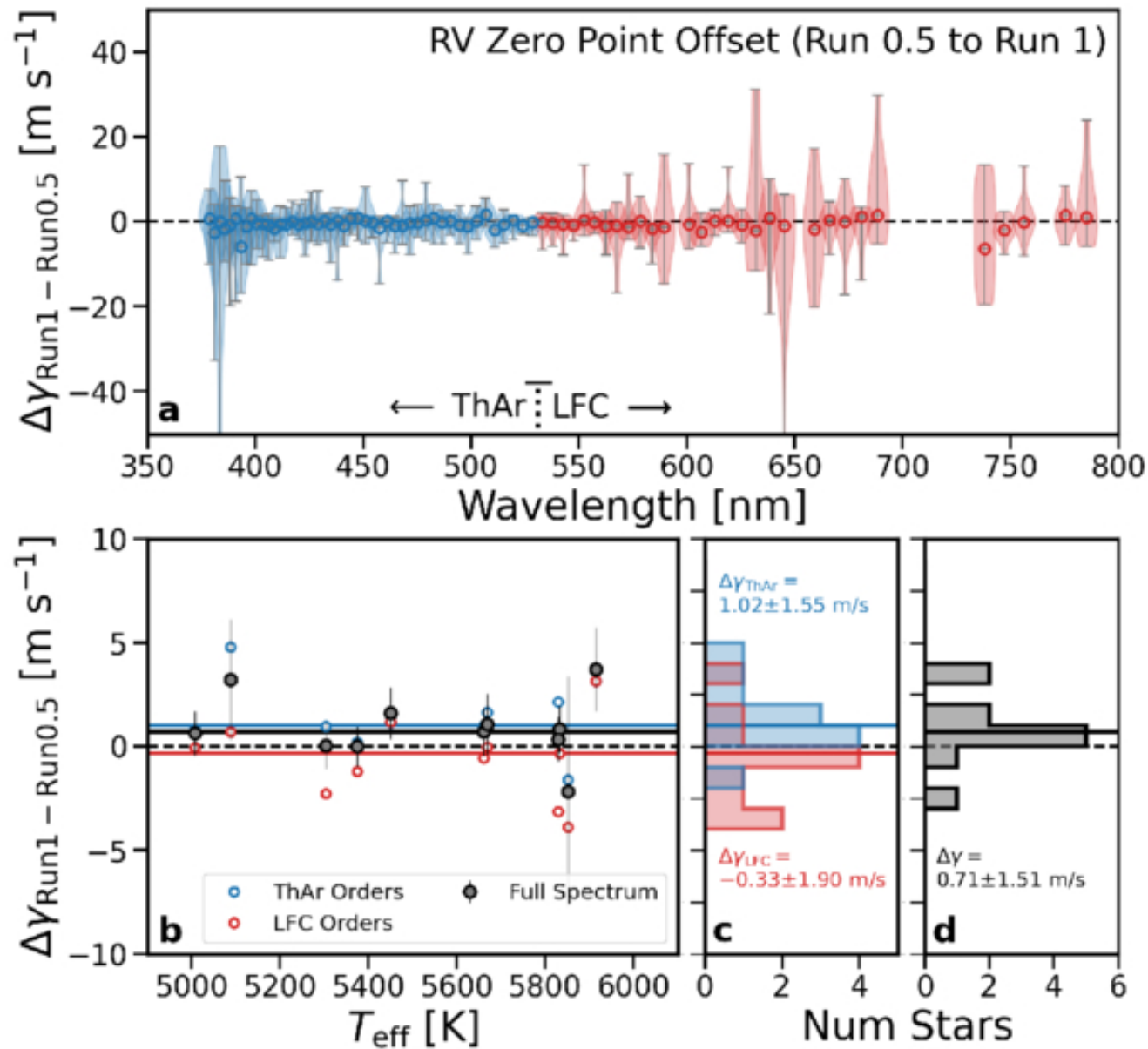
Figure 5. from Arvind F. Gupta et al 2025 Astron. J. 170 doi:10.3847/1538-3881/ae0339 https://dx.doi.org/10.3847/1538-3881/ae0339 © 2025. The Author(s). Published by the American Astronomical Society.
