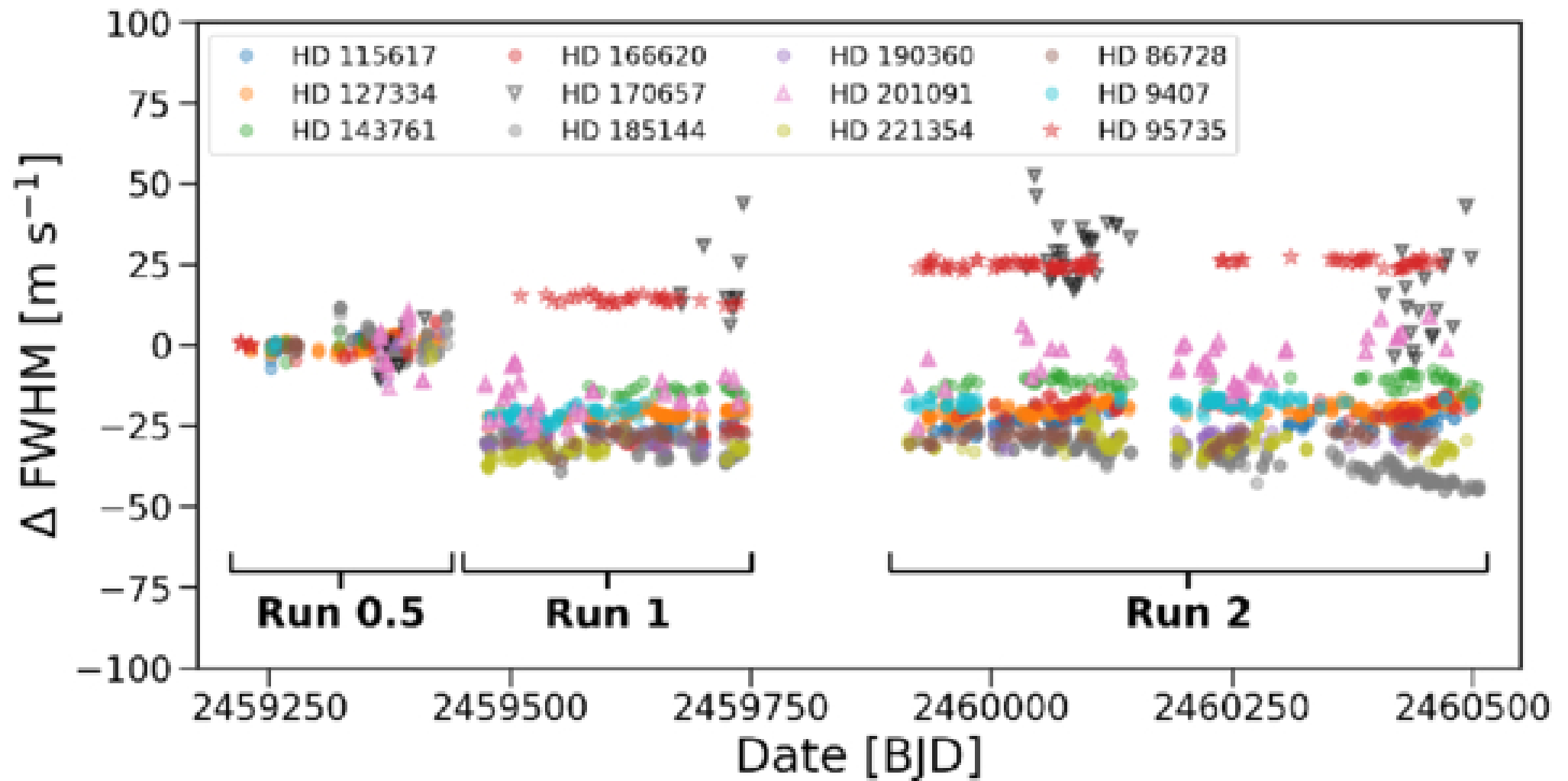
Figure 4. from Arvind F. Gupta et al 2025 Astron. J. 170 doi:10.3847/1538-3881/ae0339 https://dx.doi.org/10.3847/1538-3881/ae0339 © 2025. The Author(s). Published by the American Astronomical Society.
