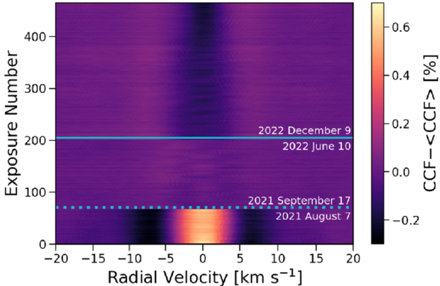
Figure 3. from Arvind F. Gupta et al 2025 Astron. J. 170 doi:10.3847/1538-3881/ae0339 https://dx.doi.org/10.3847/1538-3881/ae0339 © 2025. The Author(s). Published by the American Astronomical Society.
