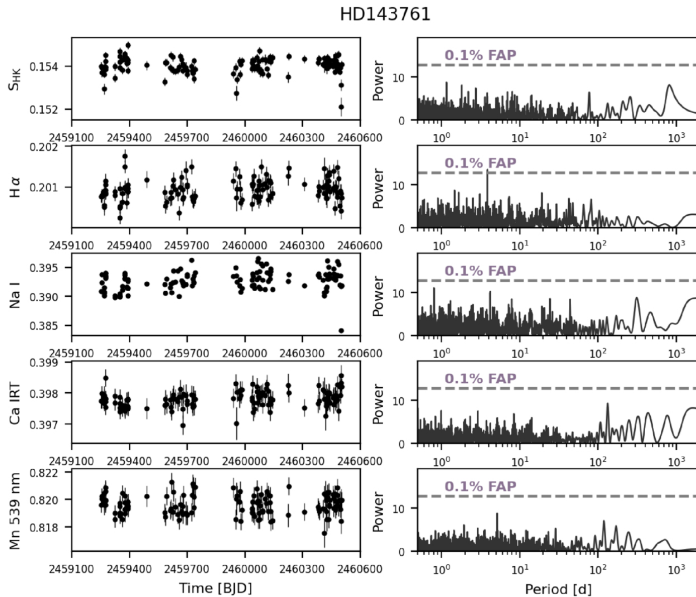
Figure 2. NEID activity indicator time series measurements and GLS periodograms. from Arvind F. Gupta et al 2025 Astron. J. 170 doi:10.3847/1538-3881/ae0339 https://dx.doi.org/10.3847/1538-3881/ae0339 © 2025. The Author(s). Published by the American Astronomical Society.
