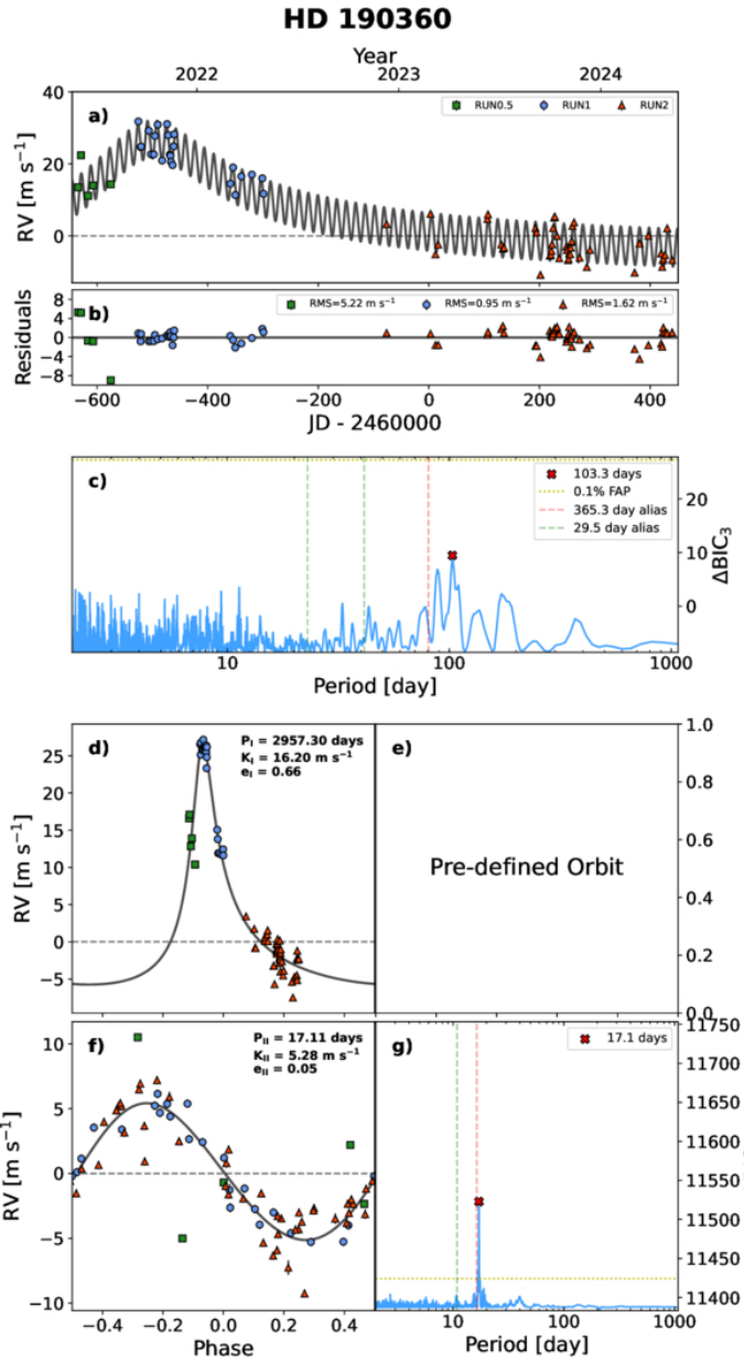
Figure 10. Informed RVSearch results for stars with known long-period companions. from Arvind F. Gupta et al 2025 Astron. J. 170 doi:10.3847/1538-3881/ae0339 https://dx.doi.org/10.3847/1538-3881/ae0339 © 2025. The Author(s). Published by the American Astronomical Society.
