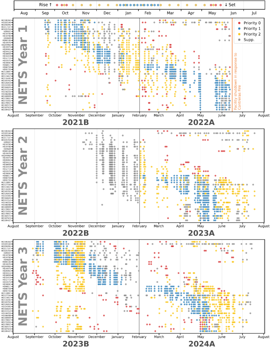
Figure 1. from Arvind F. Gupta et al 2025 Astron. J. 170 doi:10.3847/1538-3881/ae0339 https://dx.doi.org/10.3847/1538-3881/ae0339 © 2025. The Author(s). Published by the American Astronomical Society.
