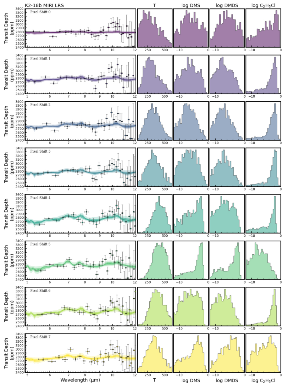
Figure 5. from Kevin B. Stevenson et al 2025 Astron. J. 170 doi:10.3847/1538-3881/ae0338 https://dx.doi.org/10.3847/1538-3881/ae0338 © 2025. The Author(s). Published by the American Astronomical Society.
