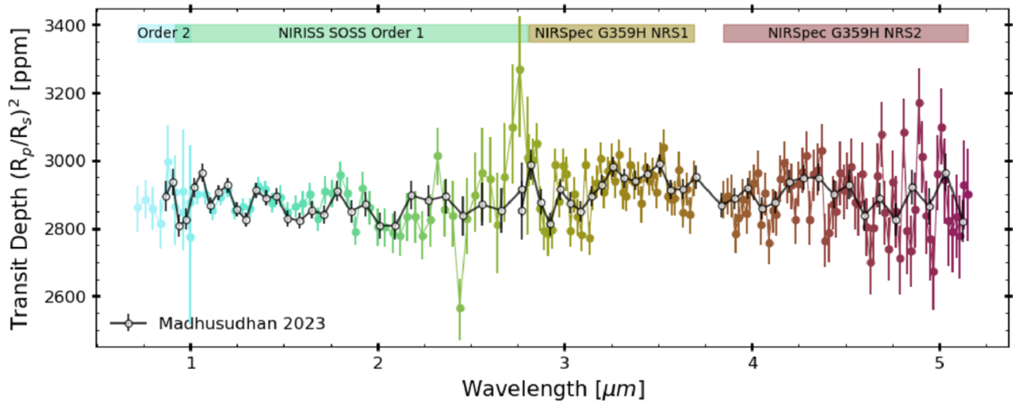
Figure 4. from Kevin B. Stevenson et al 2025 Astron. J. 170 doi:10.3847/1538-3881/ae0338 https://dx.doi.org/10.3847/1538-3881/ae0338 © 2025. The Author(s). Published by the American Astronomical Society.
