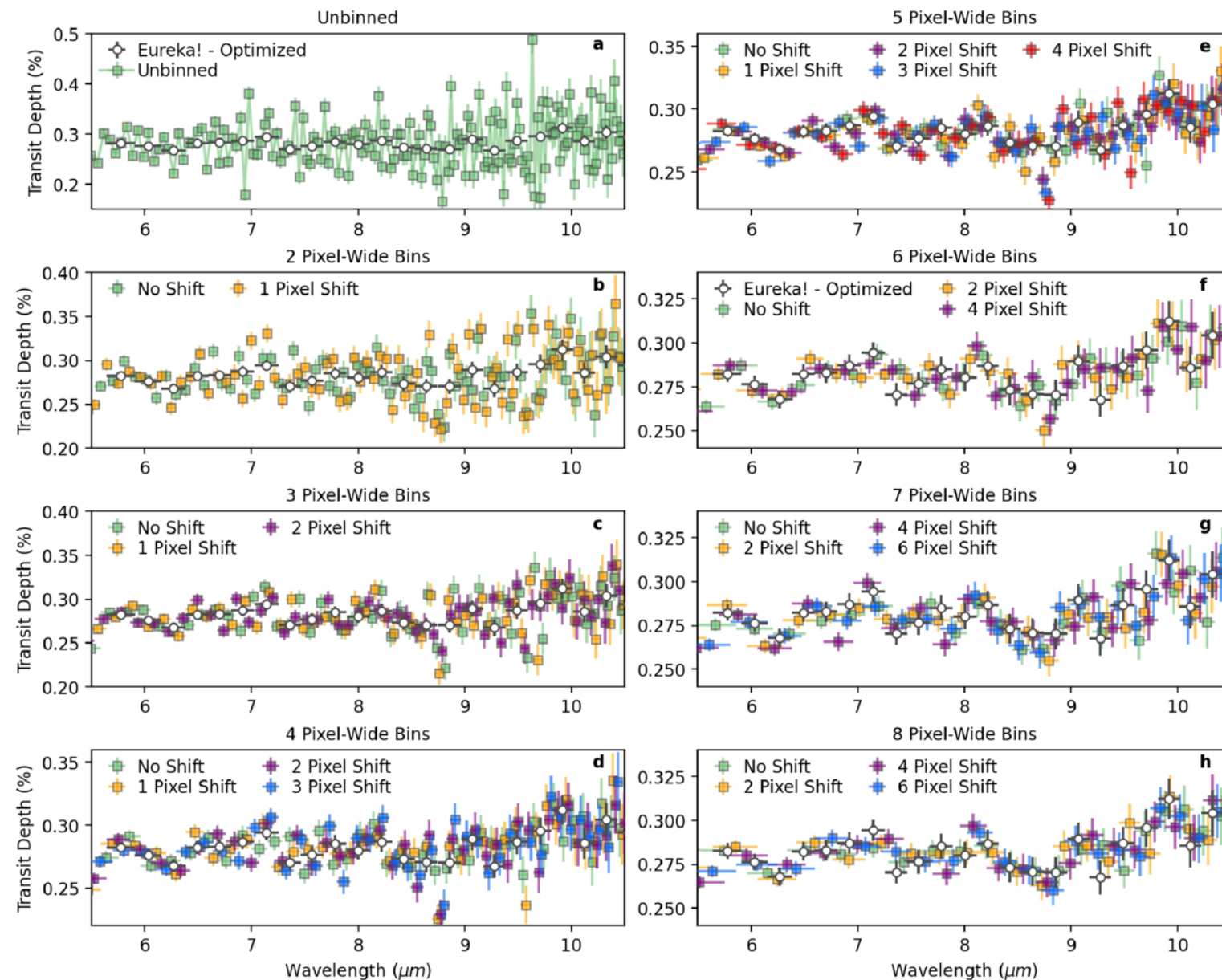
Figure 2. from Kevin B. Stevenson et al 2025 Astron. J. 170 doi:10.3847/1538-3881/ae0338 https://dx.doi.org/10.3847/1538-3881/ae0338 © 2025. The Author(s). Published by the American Astronomical Society.
