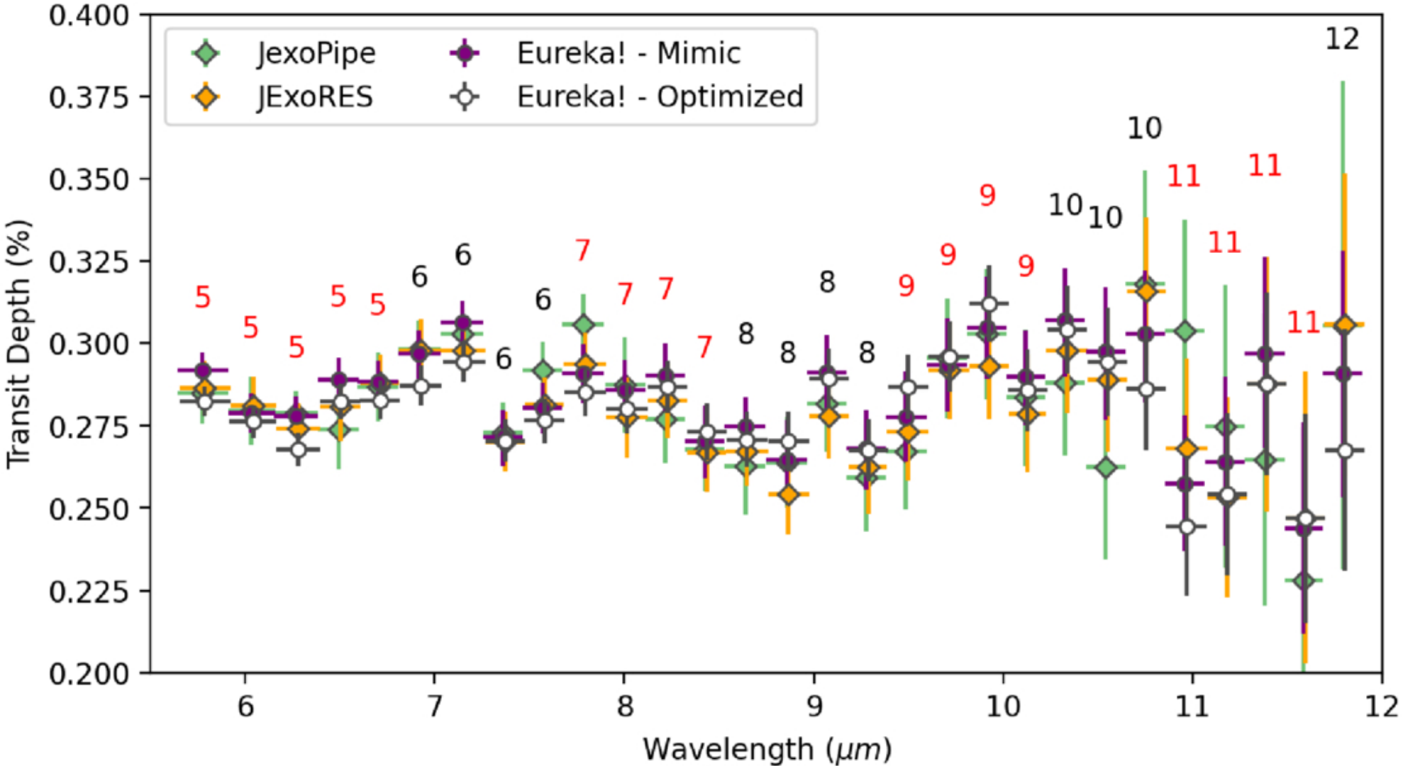
Figure 1. from Kevin B. Stevenson et al 2025 Astron. J. 170 doi:10.3847/1538-3881/ae0338 https://dx.doi.org/10.3847/1538-3881/ae0338 © 2025. The Author(s). Published by the American Astronomical Society.
