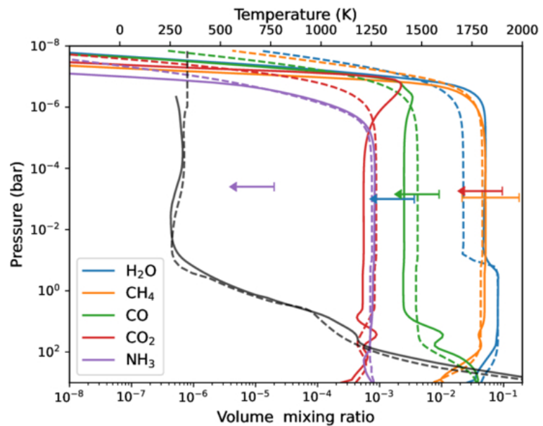
Figure 9. from Stephen P. Schmidt et al 2025 Astron. J. 170 doi:10.3847/1538-3881/ae019a https://dx.doi.org/10.3847/1538-3881/ae019a © 2025. The Author(s). Published by the American Astronomical Society.
