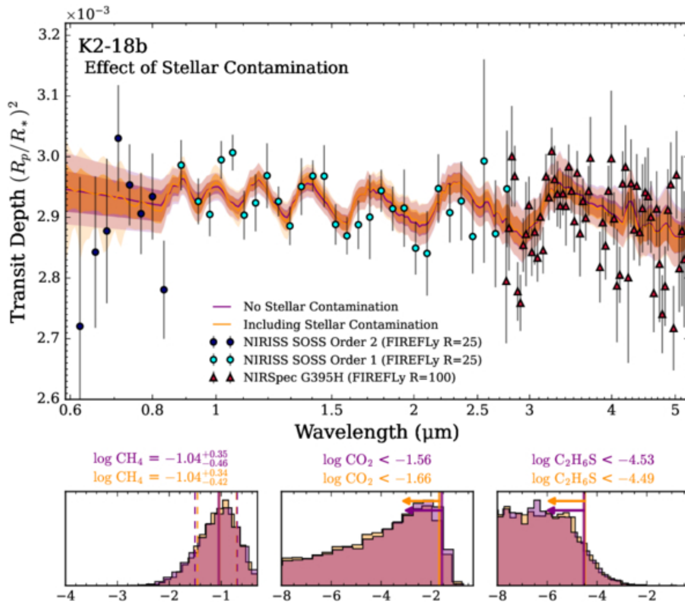
Figure 8. from Stephen P. Schmidt et al 2025 Astron. J. 170 doi:10.3847/1538-3881/ae019a https://dx.doi.org/10.3847/1538-3881/ae019a © 2025. The Author(s). Published by the American Astronomical Society.
