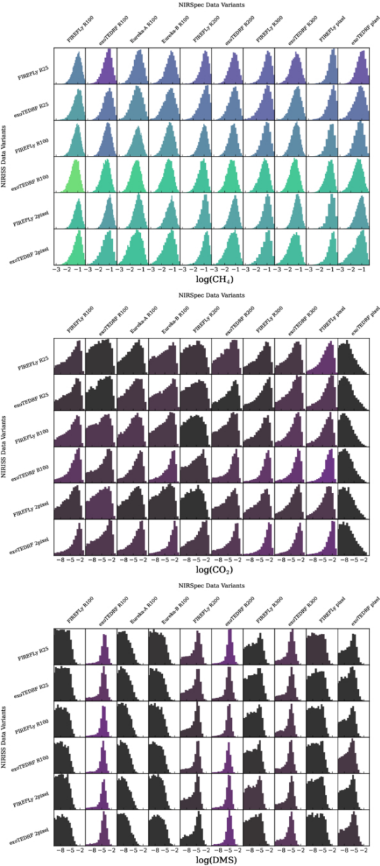
Figure 7. from Stephen P. Schmidt et al 2025 Astron. J. 170 doi:10.3847/1538-3881/ae019a https://dx.doi.org/10.3847/1538-3881/ae019a © 2025. The Author(s). Published by the American Astronomical Society.
