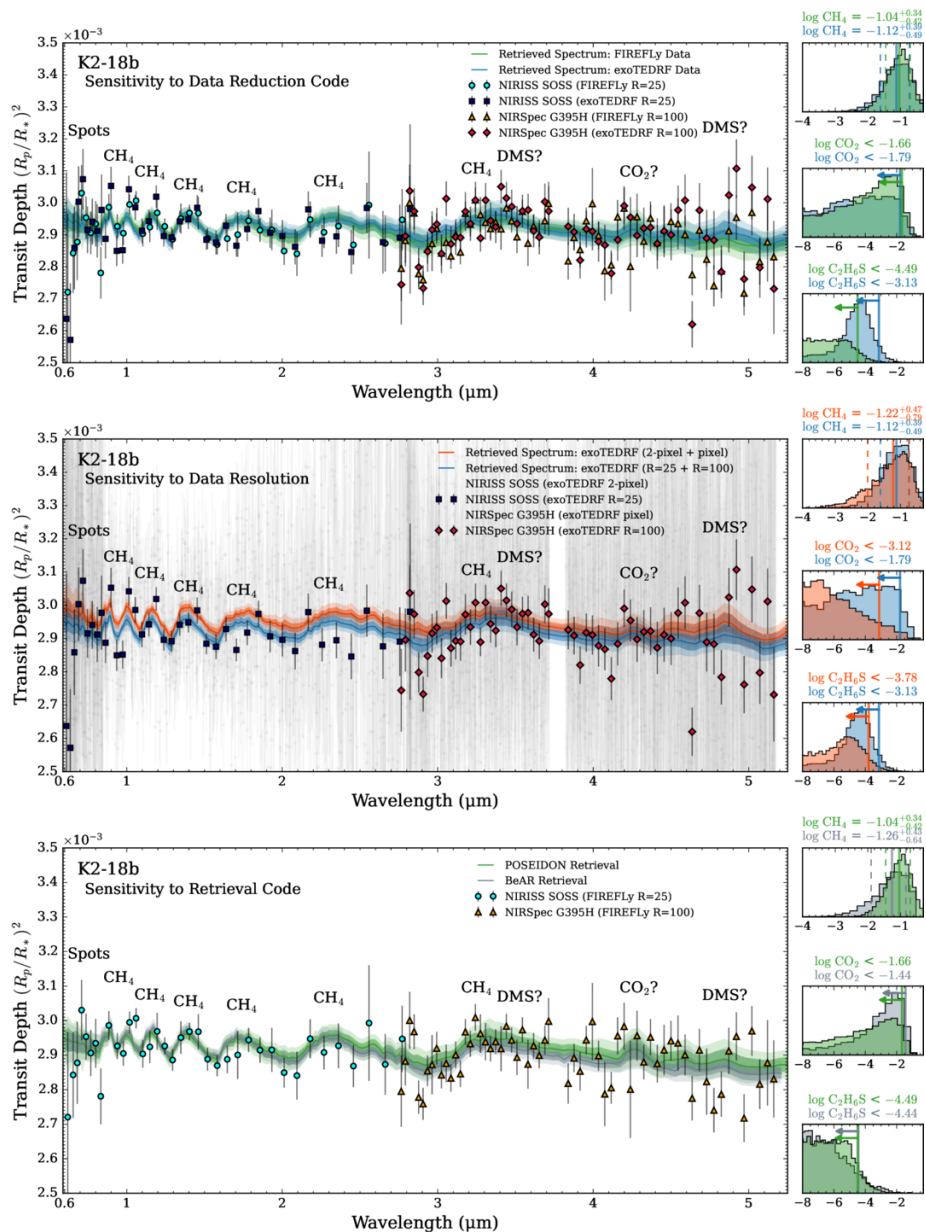
Figure 6. from Stephen P. Schmidt et al 2025 Astron. J. 170 doi:10.3847/1538-3881/ae019a https://dx.doi.org/10.3847/1538-3881/ae019a © 2025. The Author(s). Published by the American Astronomical Society.
