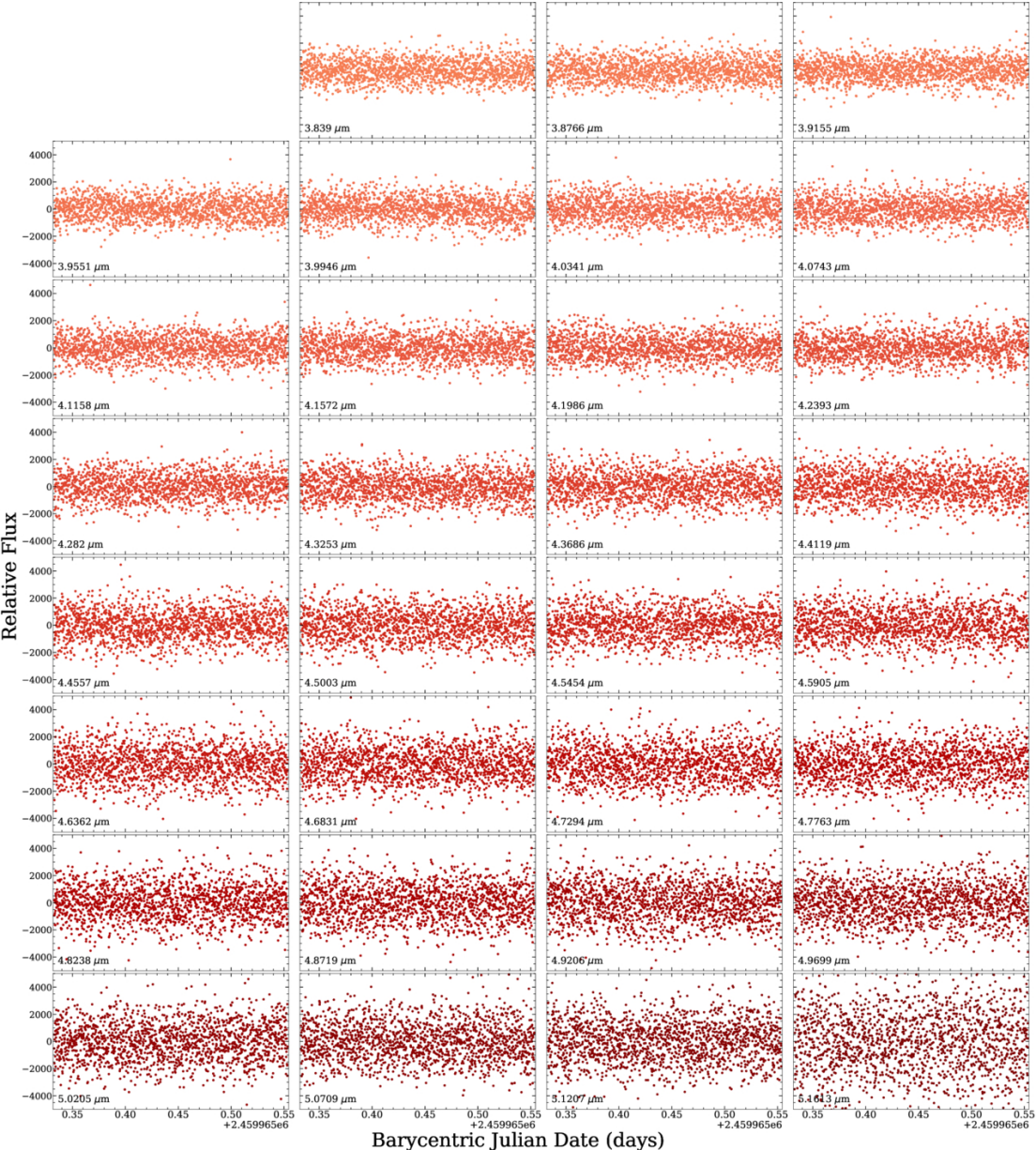
Figure 20. from Stephen P. Schmidt et al 2025 Astron. J. 170 doi:10.3847/1538-3881/ae019a https://dx.doi.org/10.3847/1538-3881/ae019a © 2025. The Author(s). Published by the American Astronomical Society.
