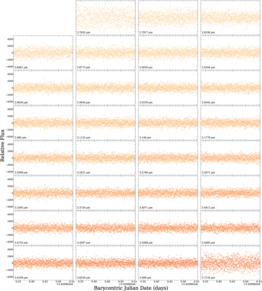
Figure 19. from Stephen P. Schmidt et al 2025 Astron. J. 170 doi:10.3847/1538-3881/ae019a https://dx.doi.org/10.3847/1538-3881/ae019a © 2025. The Author(s). Published by the American Astronomical Society.
