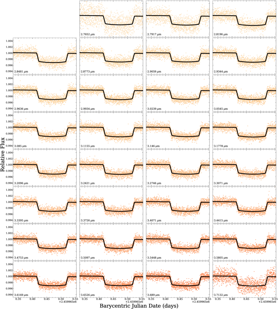
Figure 17. from Stephen P. Schmidt et al 2025 Astron. J. 170 doi:10.3847/1538-3881/ae019a https://dx.doi.org/10.3847/1538-3881/ae019a © 2025. The Author(s). Published by the American Astronomical Society.
