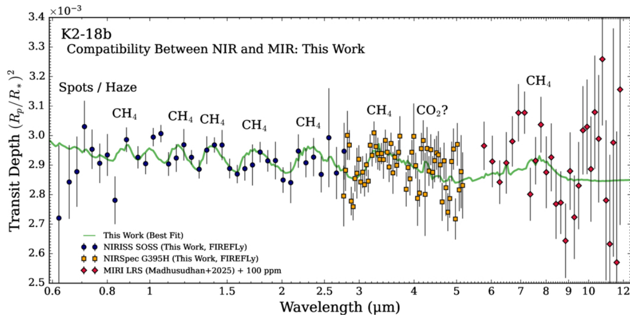
Figure 14. from Stephen P. Schmidt et al 2025 Astron. J. 170 doi:10.3847/1538-3881/ae019a https://dx.doi.org/10.3847/1538-3881/ae019a © 2025. The Author(s). Published by the American Astronomical Society.
