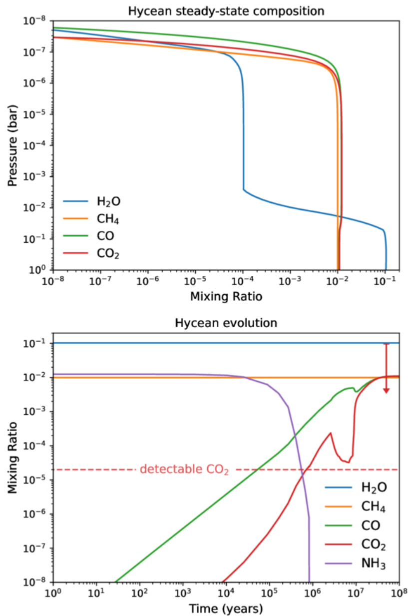
Figure 12. from Stephen P. Schmidt et al 2025 Astron. J. 170 doi:10.3847/1538-3881/ae019a https://dx.doi.org/10.3847/1538-3881/ae019a © 2025. The Author(s). Published by the American Astronomical Society.
