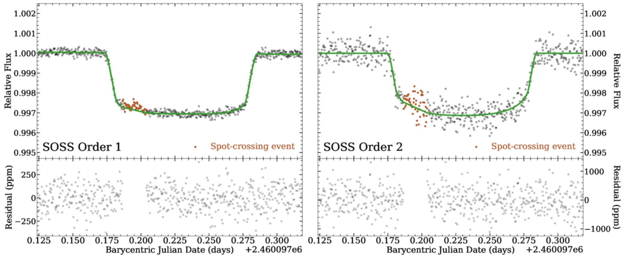
Figure 1. from Stephen P. Schmidt et al 2025 Astron. J. 170 doi:10.3847/1538-3881/ae019a https://dx.doi.org/10.3847/1538-3881/ae019a © 2025. The Author(s). Published by the American Astronomical Society.
