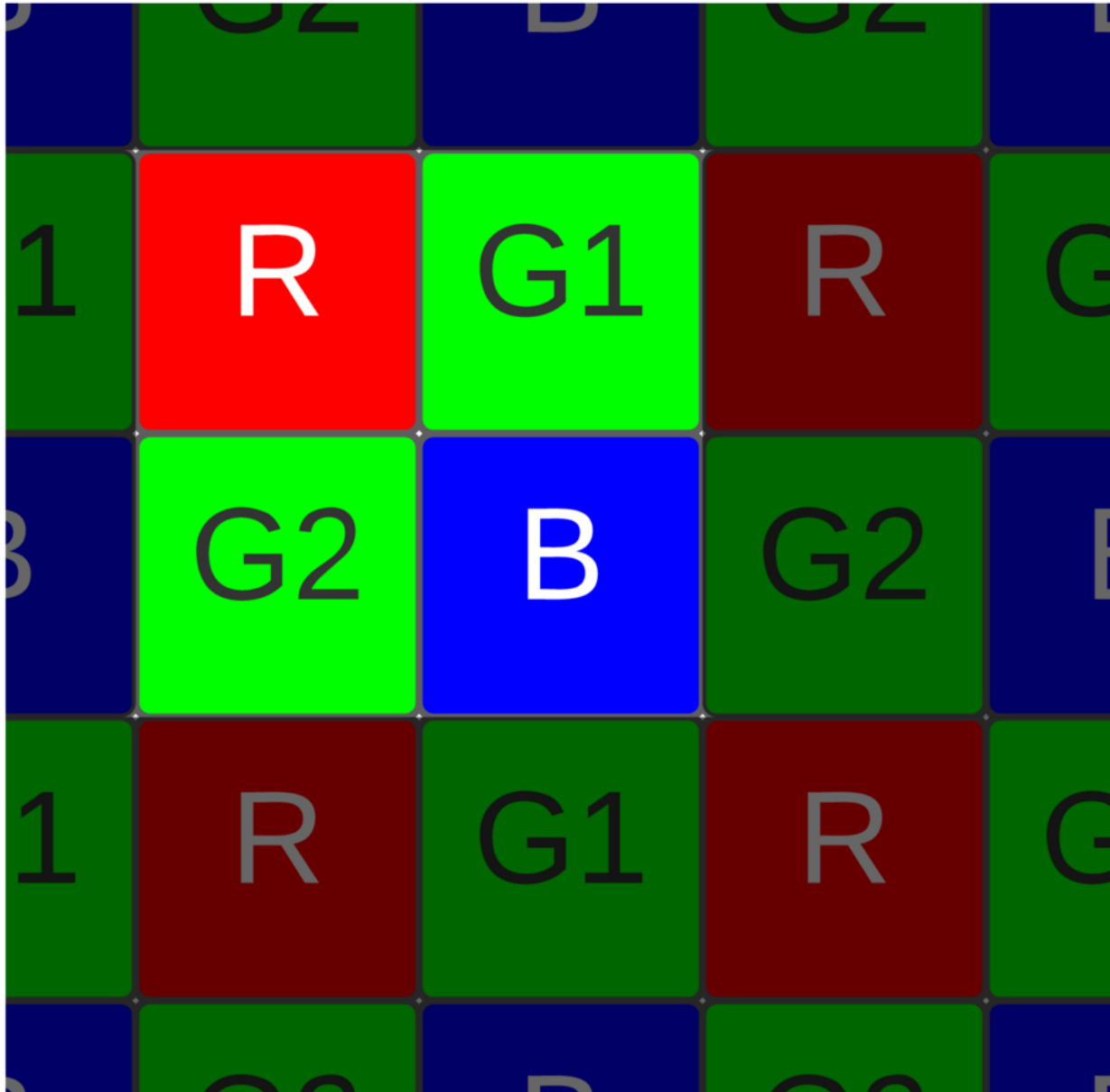
Figure 2. from Angel E. Romero et al 2025 Astron. J. 170 doi:10.3847/1538-3881/adfe6c https://dx.doi.org/10.3847/1538-3881/adfe6c © 2025. The Author(s). Published by the American Astronomical Society.
