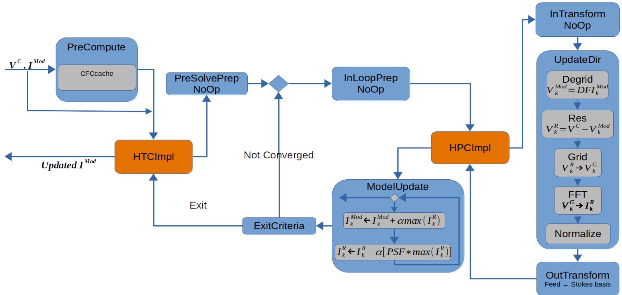
S. Bhatnagar et al 2025 Astron. J. 170 doi:10.3847/1538-3881/adfe61 https://dx.doi.org/10.3847/1538-3881/adfe61 © 2025. The Author(s). Published by the American Astronomical Society.
