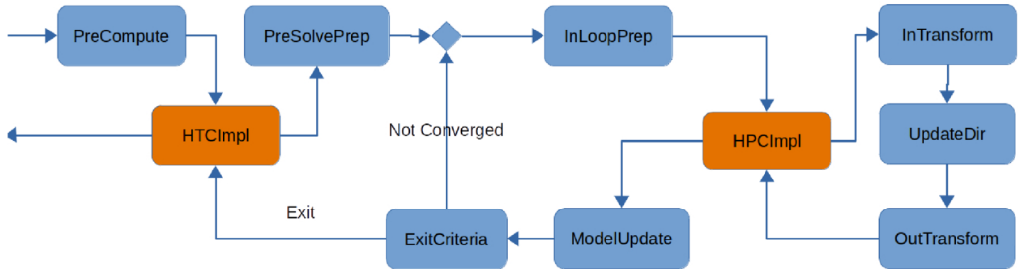
Figure 3. from S. Bhatnagar et al 2025 Astron. J. 170 doi:10.3847/1538-3881/adfe61 https://dx.doi.org/10.3847/1538-3881/adfe61 © 2025. The Author(s). Published by the American Astronomical Society.
