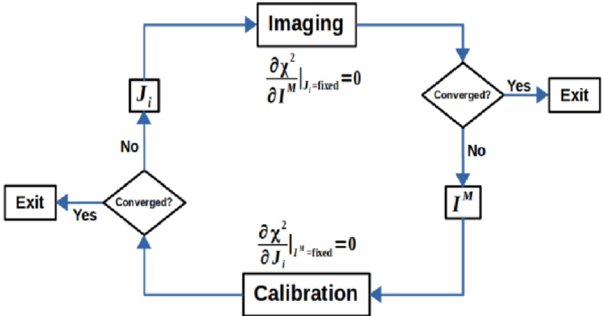
Figure 2. from S. Bhatnagar et al 2025 Astron. J. 170 doi:10.3847/1538-3881/adfe61 https://dx.doi.org/10.3847/1538-3881/adfe61 © 2025. The Author(s). Published by the American Astronomical Society.
