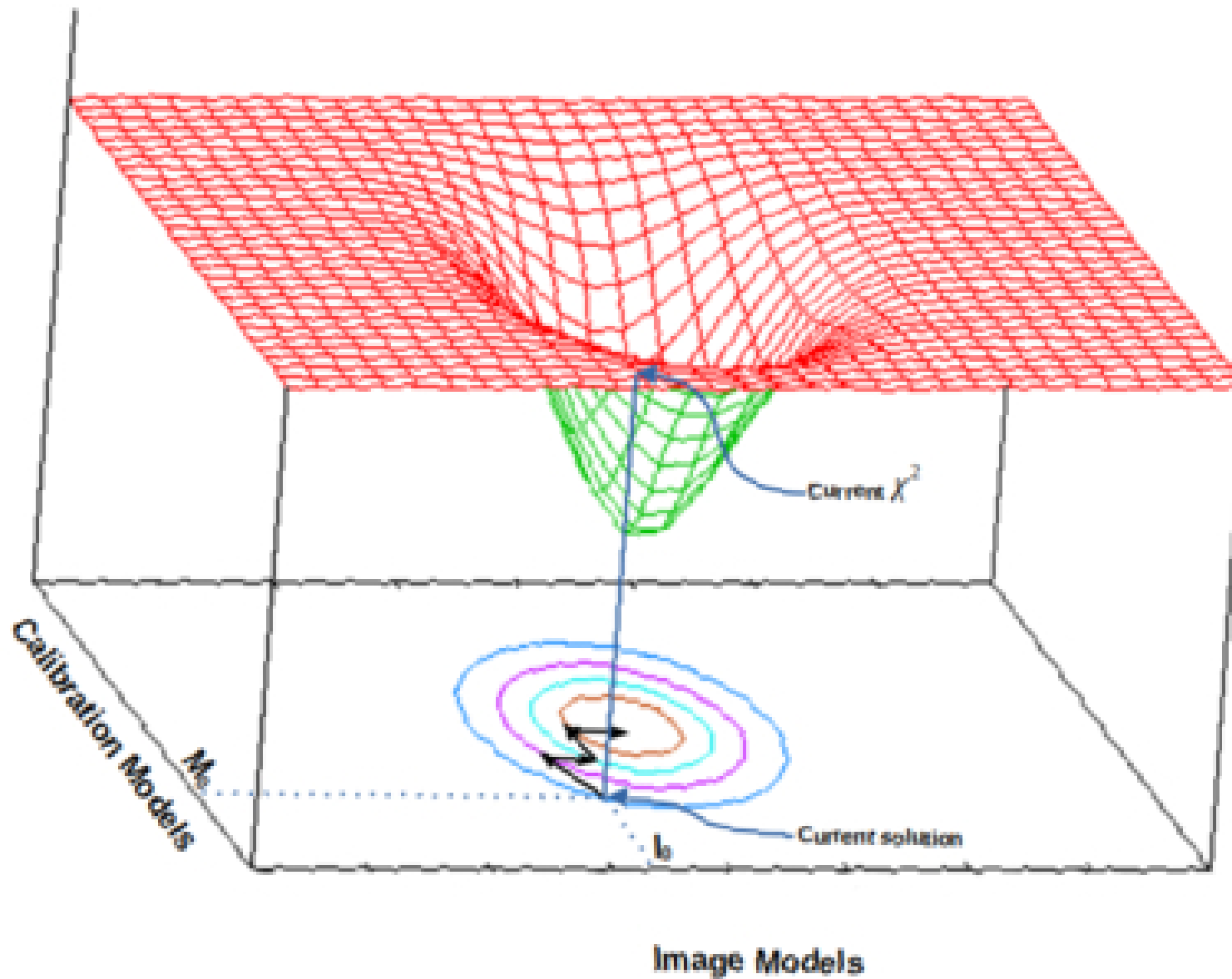
Figure 1. from S. Bhatnagar et al 2025 Astron. J. 170 doi:10.3847/1538-3881/adfe61 https://dx.doi.org/10.3847/1538-3881/adfe61 © 2025. The Author(s). Published by the American Astronomical Society.
