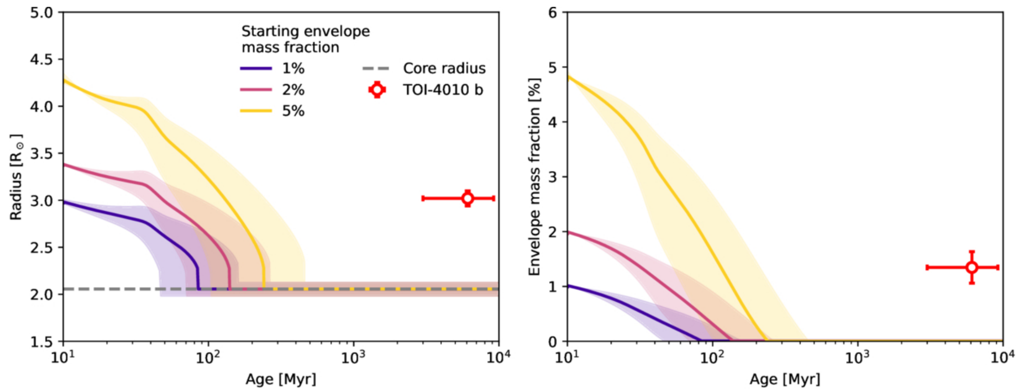
Figure 8. from Morgan Saidel et al 2025 Astron. J. 170 doi:10.3847/1538-3881/adfe5e https://dx.doi.org/10.3847/1538-3881/adfe5e © 2025. The Author(s). Published by the American Astronomical Society.
