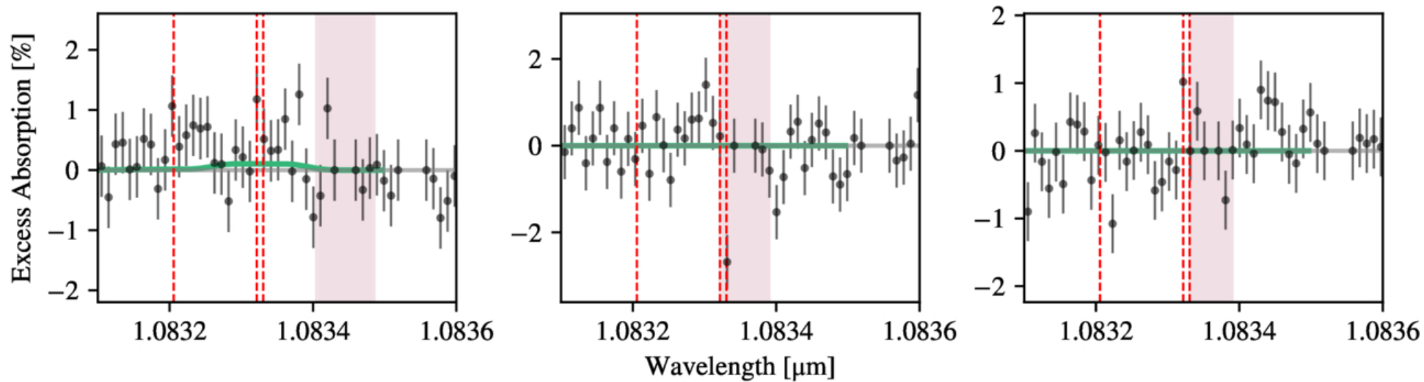
Figure 6. from Morgan Saidel et al 2025 Astron. J. 170 doi:10.3847/1538-3881/adfe5e https://dx.doi.org/10.3847/1538-3881/adfe5e © 2025. The Author(s). Published by the American Astronomical Society.
