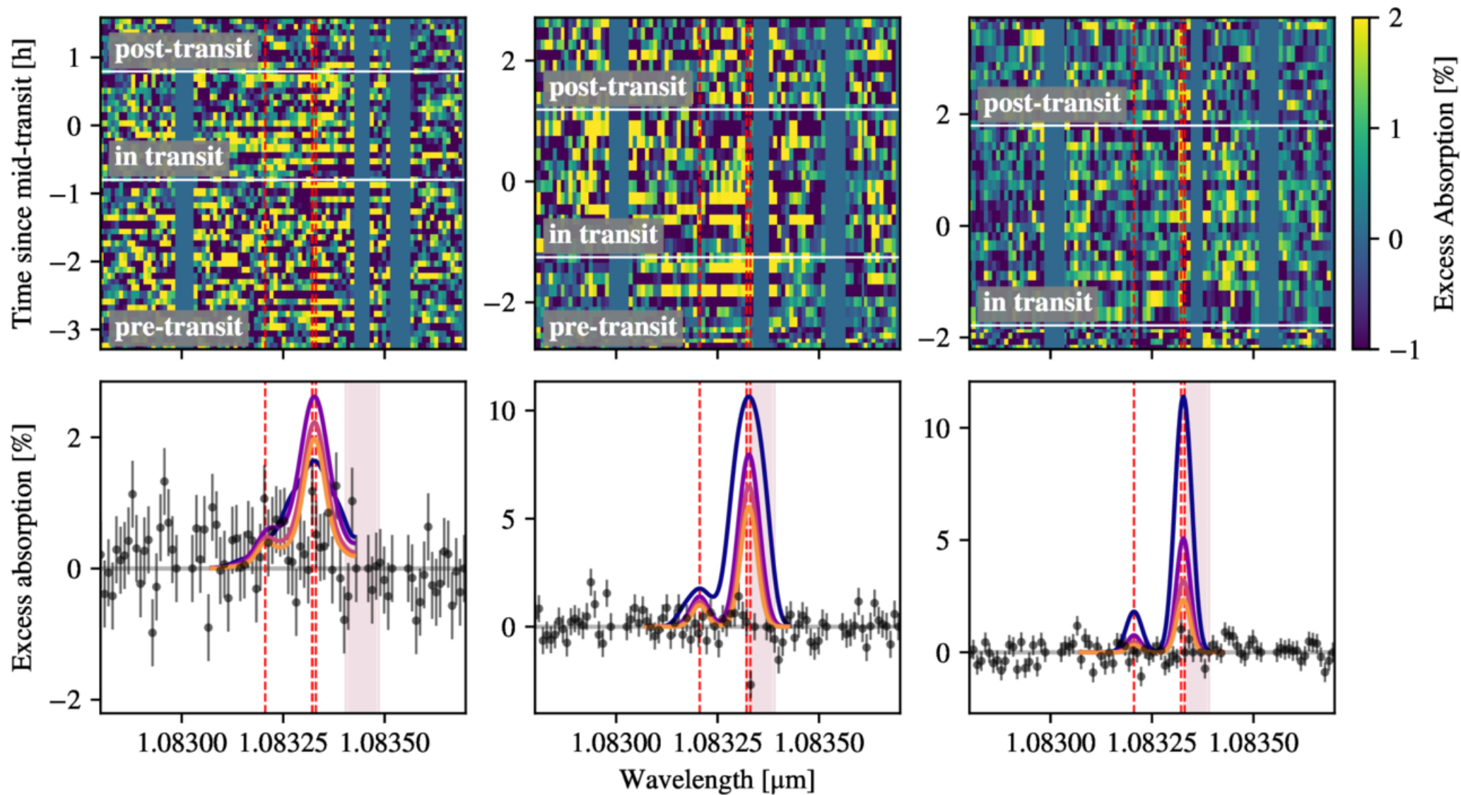
Figure 3. from Morgan Saidel et al 2025 Astron. J. 170 doi:10.3847/1538-3881/adfe5e https://dx.doi.org/10.3847/1538-3881/adfe5e © 2025. The Author(s). Published by the American Astronomical Society.
