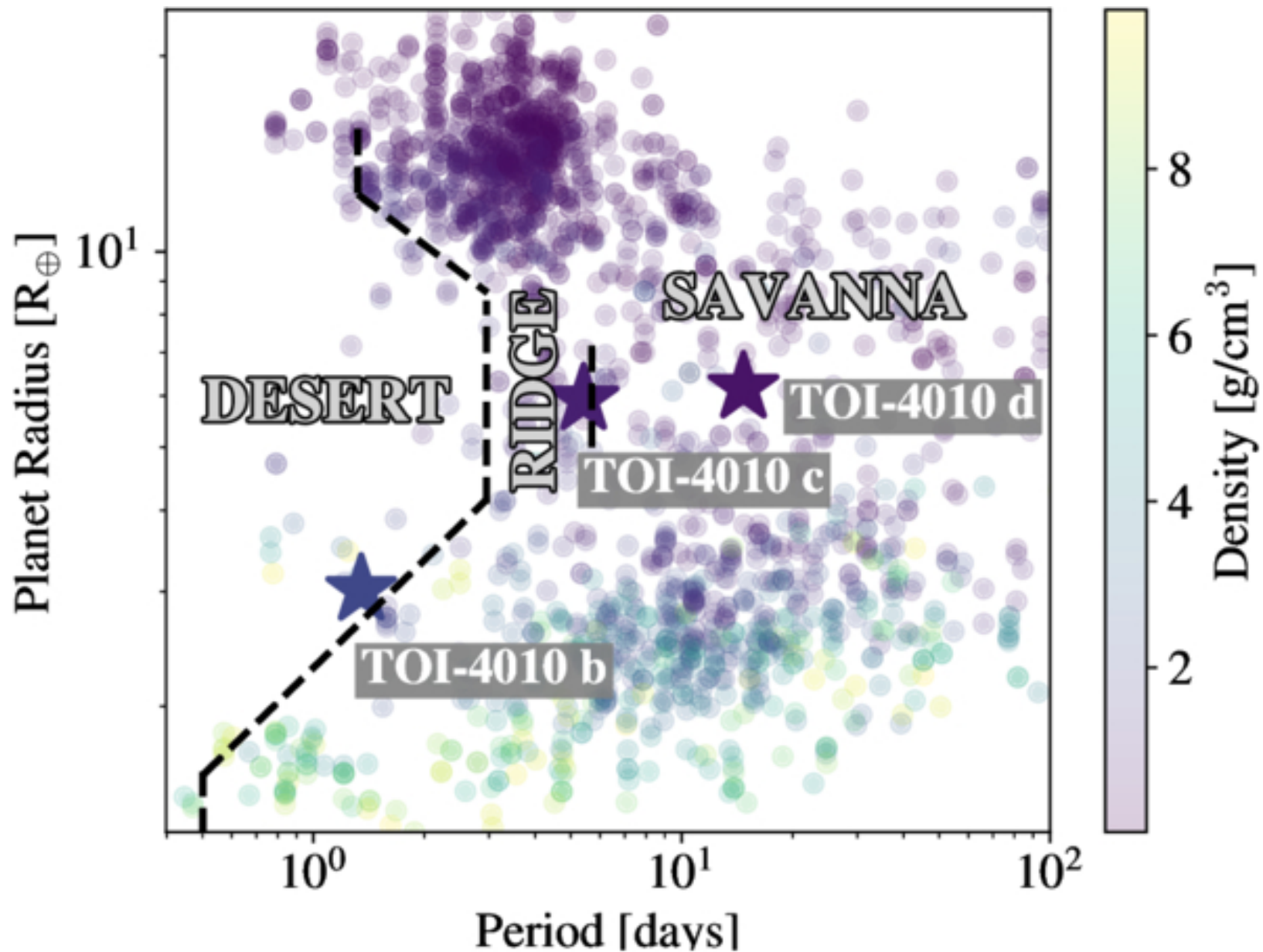
Figure 1. from Morgan Sidel et al 2025 Astron. J. 170 doi:10.3847/1538-3881/adfe5e https://dx.doi.org/10.3847/1538-3881/adfe5e © 2025. The Author(s). Published by the American Astronomical Society.
