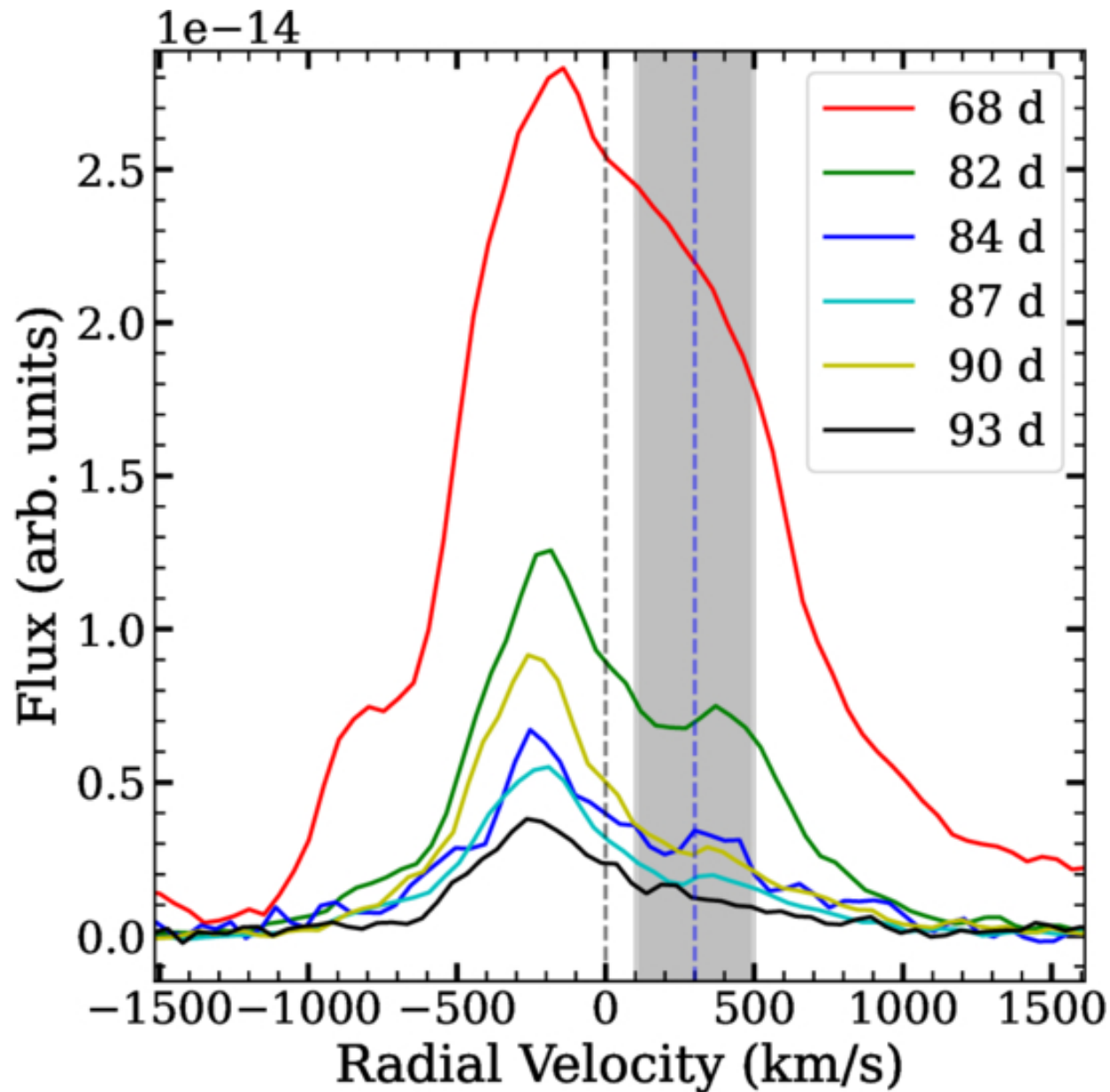
Figure 8. from Mohit Singh Bisht et al 2025 Astron. J. 170 doi:10.3847/1538-3881/adfcc6 https://dx.doi.org/10.3847/1538-3881/adfcc6 © 2025. The Author(s). Published by the American Astronomical Society.
