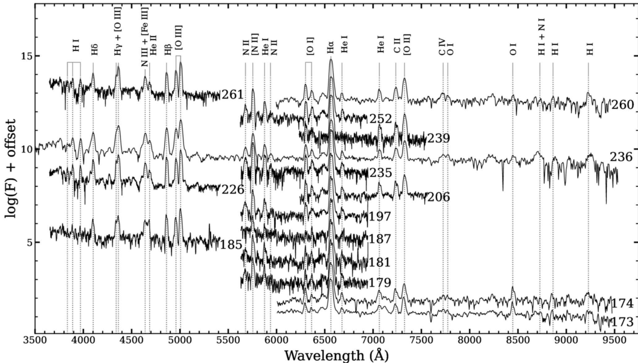
Figure 7. from Mohit Singh Bisht et al 2025 Astron. J. 170 doi:10.3847/1538-3881/adfcc6 https://dx.doi.org/10.3847/1538-3881/adfcc6 © 2025. The Author(s). Published by the American Astronomical Society.
