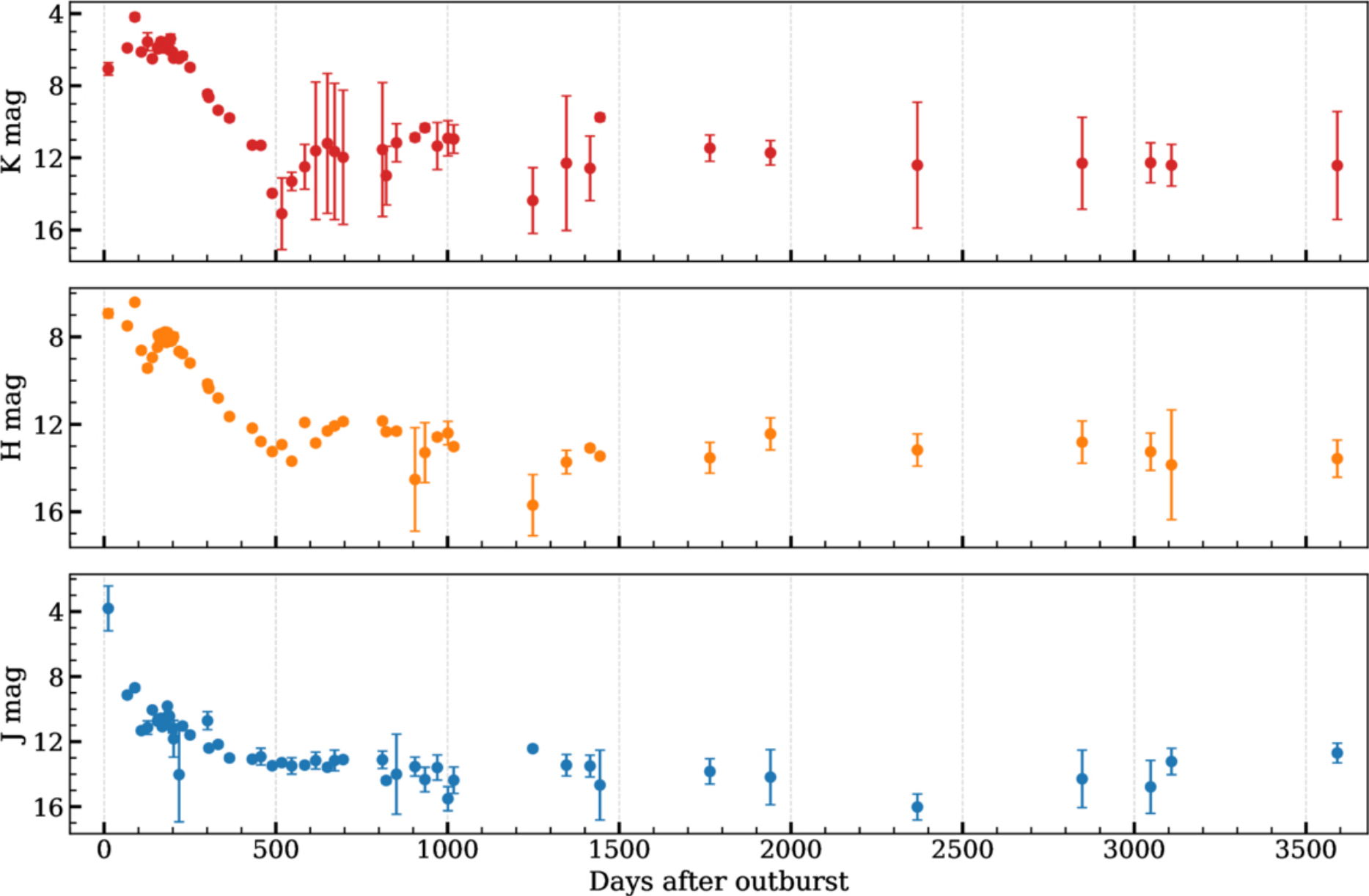
Figure 3. from Mohit Singh Bisht et al 2025 Astron. J. 170 doi:10.3847/1538-3881/adfcc6 https://dx.doi.org/10.3847/1538-3881/adfcc6 © 2025. The Author(s). Published by the American Astronomical Society.
