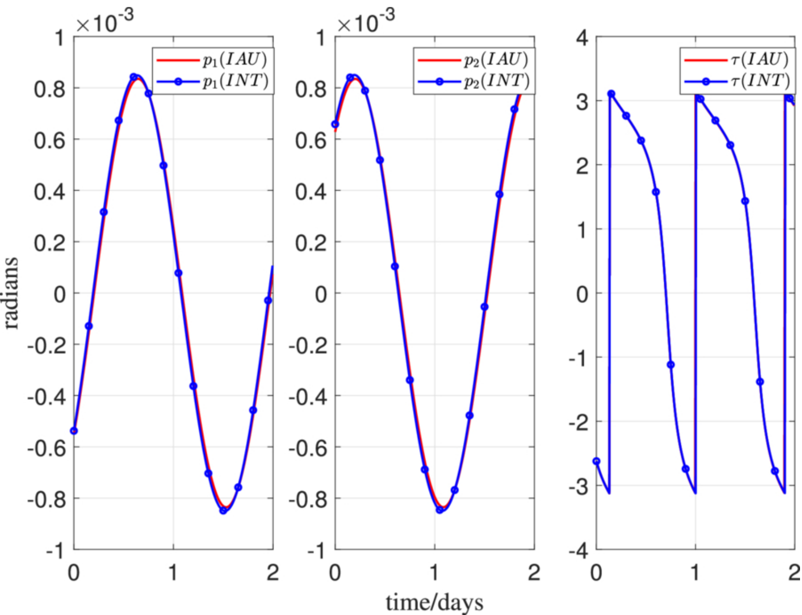
Figure 8. from Lidan Zhang et al 2025 Astron. J. 170 doi:10.3847/1538-3881/adfc54 https://dx.doi.org/10.3847/1538-3881/adfc54 © 2025. The Author(s). Published by the American Astronomical Society.
